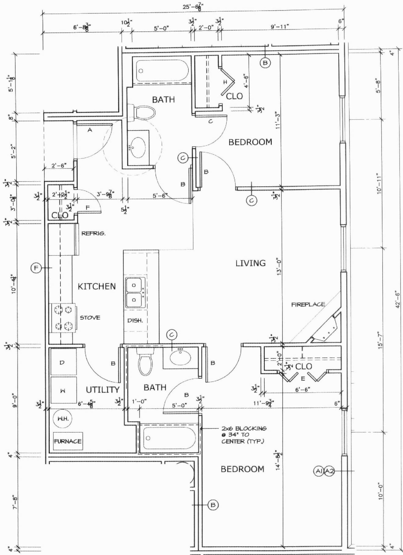
ENLARGED UNIT PLAN 'D'
