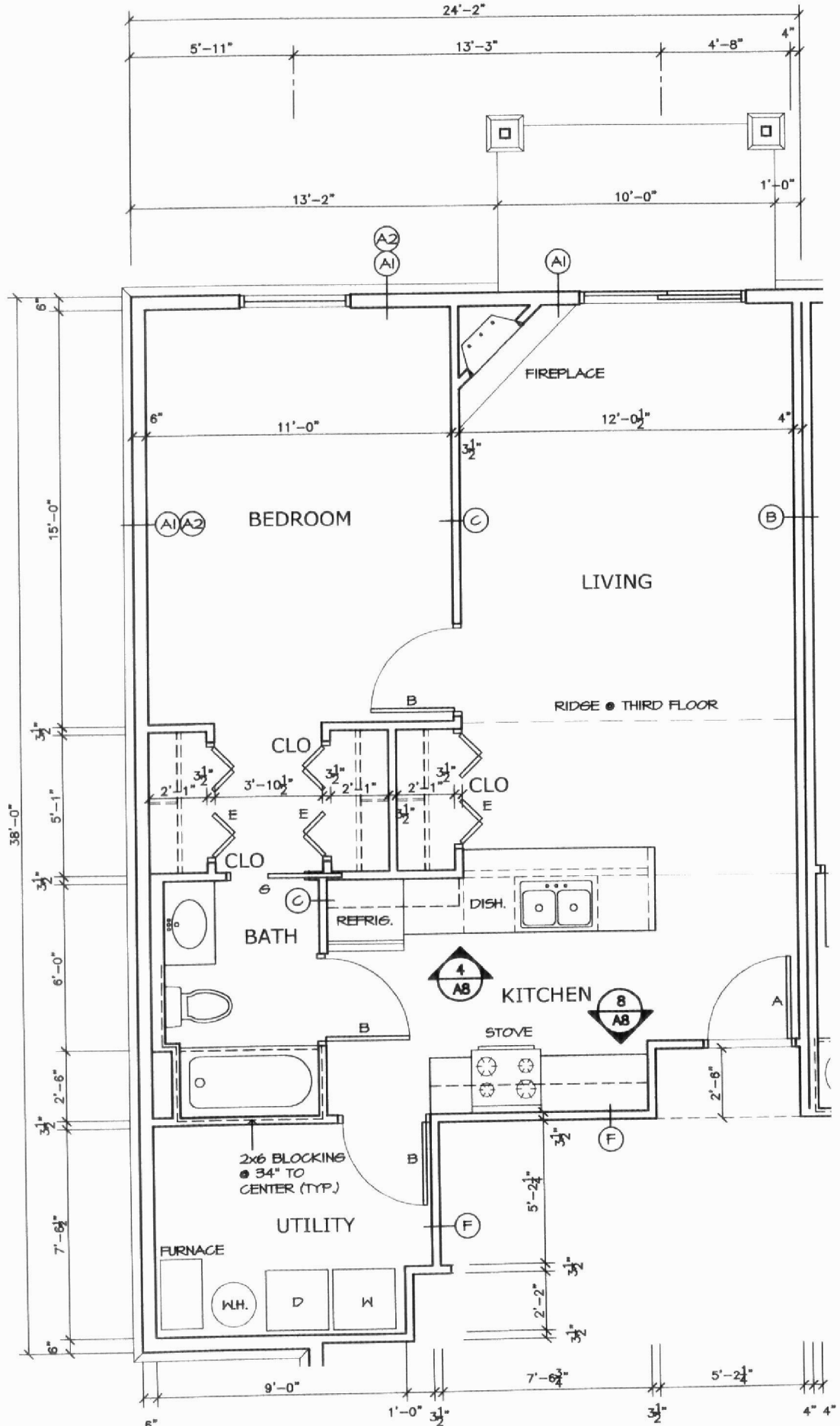
ENLARGED UNIT PLAN 'C' 1/4" = 1'-0"
