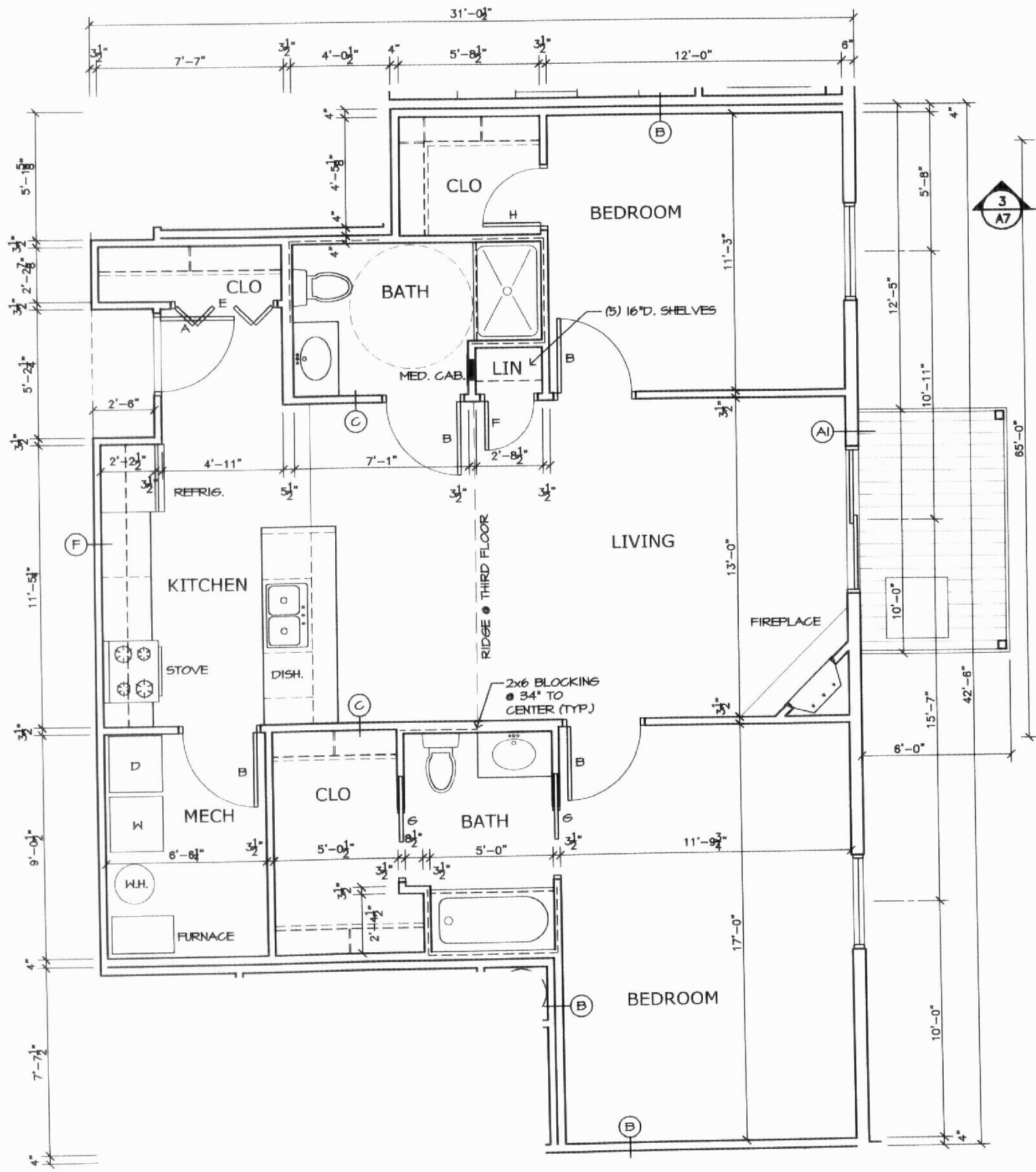
ENLARGED UNIT PLAN 'E' 1/4" = 1'-0" ACCESSIBLE TYPE 'A' UNIT
